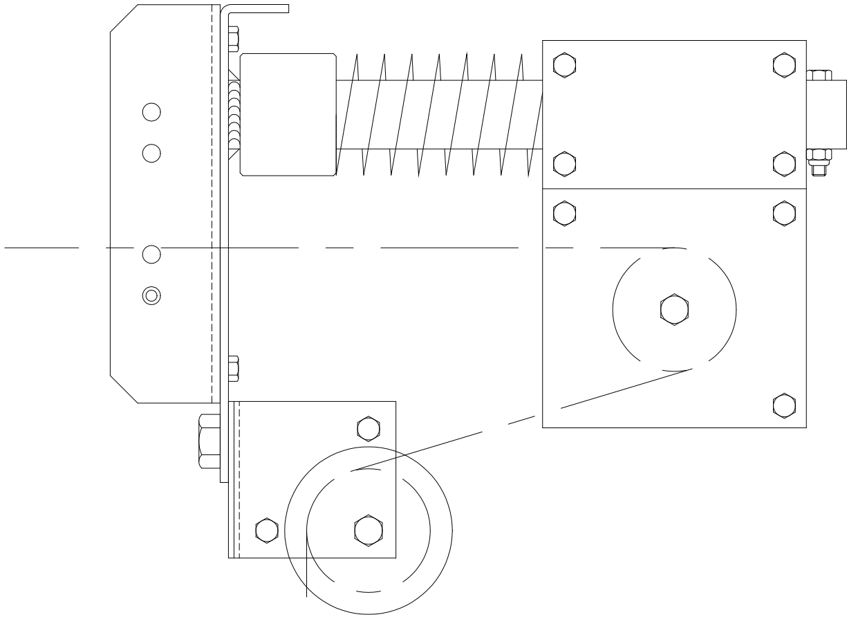
SPRING HEAD PULLEY STA-12
