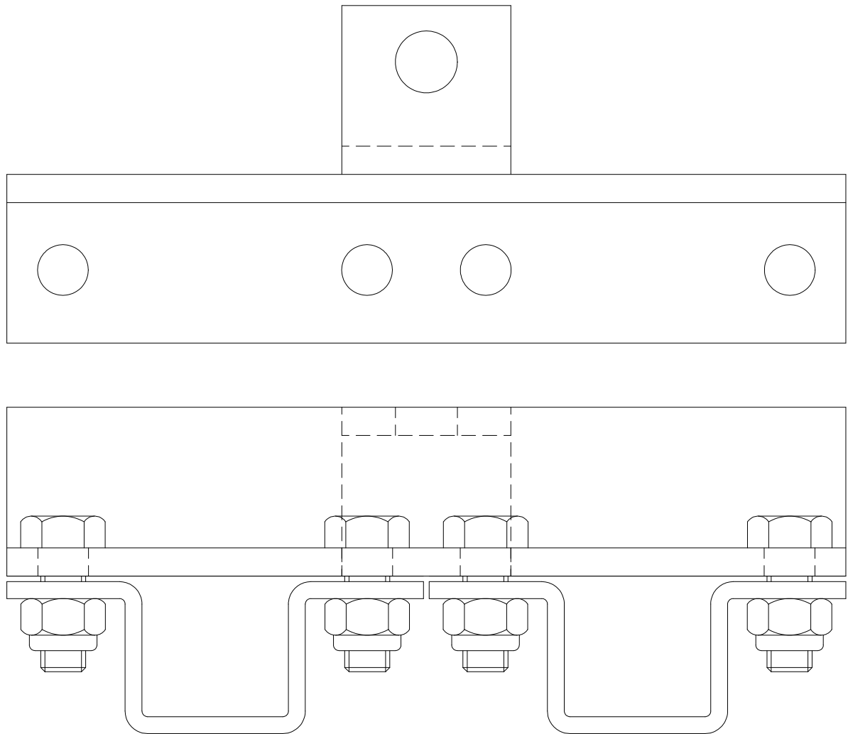
OVERLAP BRACKET STB-13
