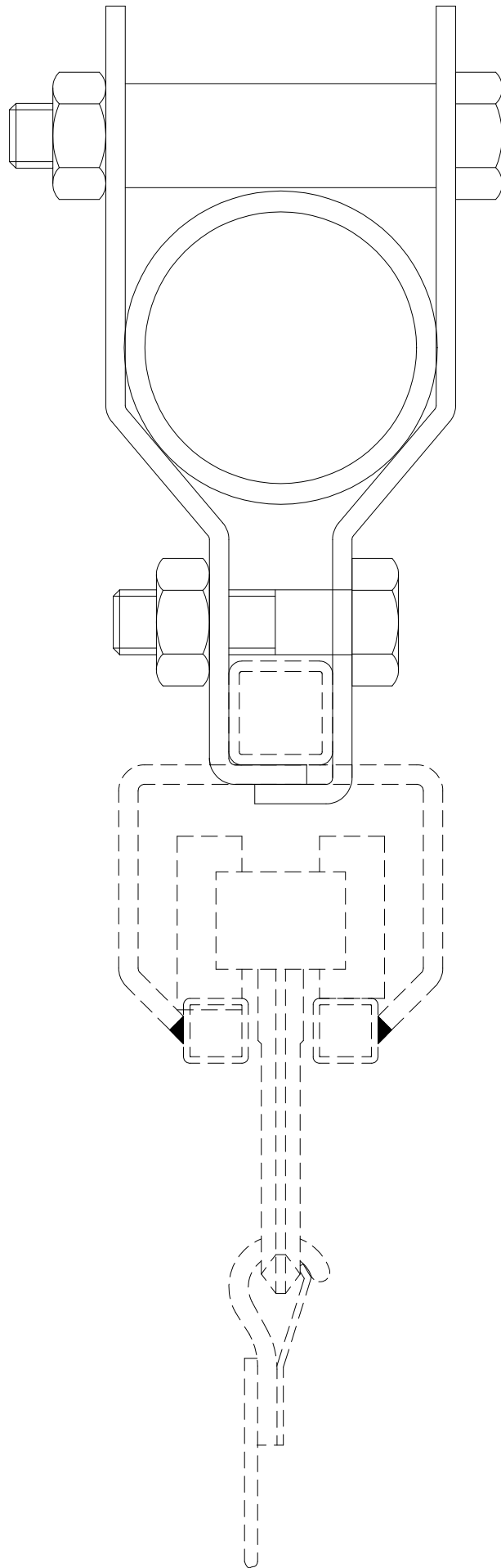
BARREL SUSPENSION STA-23
